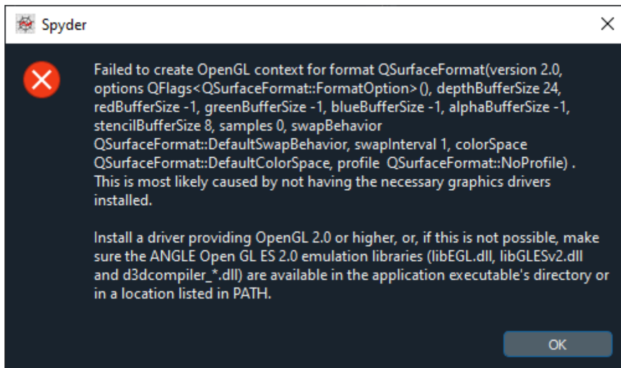
Figure 14: OpenGL error
