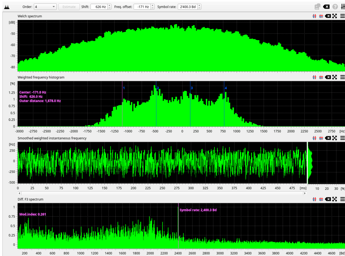
Figure 39: FSK analysis result display overview (FSK-4).
