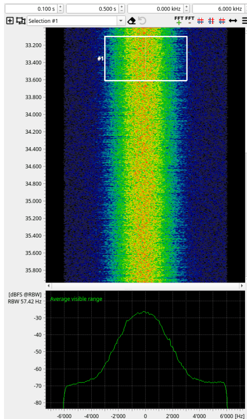
Figure 38: Input sonogram of the FSK-4 example.
