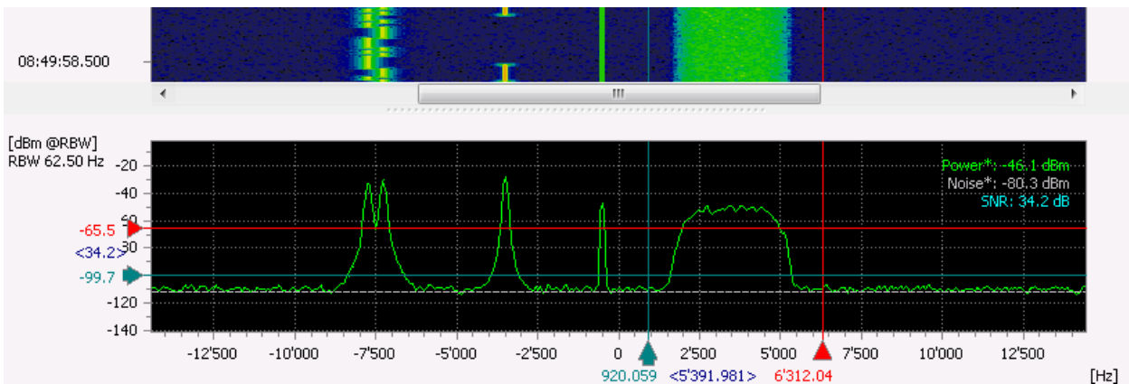
Figure 15: Spectrum/Sonogram with manually positioned Y-cursor
