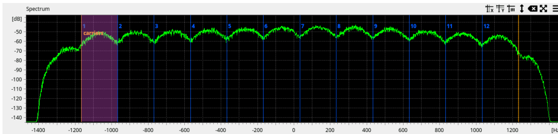
Figure 41: Averaged spectrum with cursors placed between carriers.
