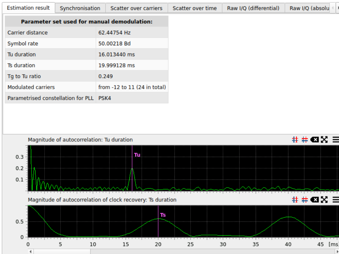
Figure 44: Results of estimation of basic OFDM parameters.
