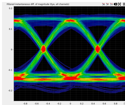
Figure 62: Eye pattern diagram for FSK-2
