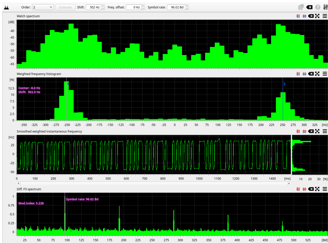
Figure 32: FSK analysis result display overview (FSK-2).
