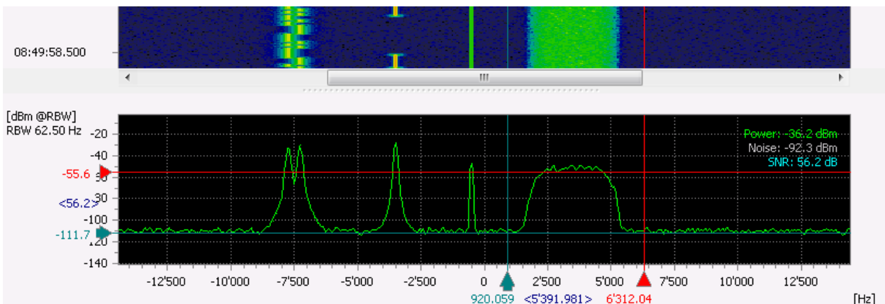
Figure 14: Spectrum/Sonogram with synchronized Y-cursor
