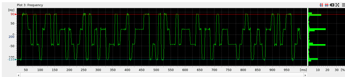
Figure 18: Frequency plot of a FSK4 emission
