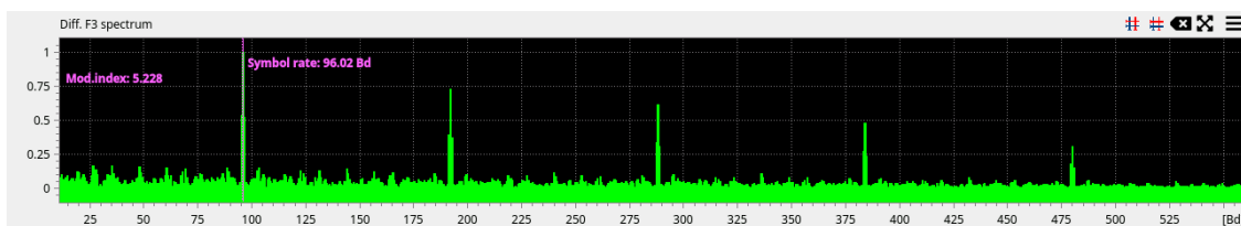
Figure 36: Diff. F3 spectrum for symbol rate estimation.
