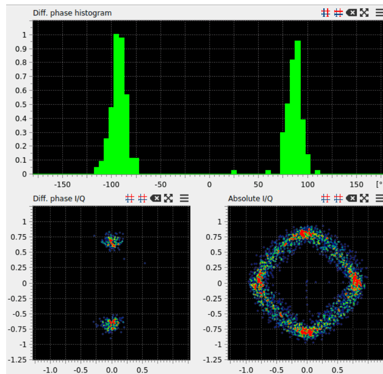
Figure 31: Differential phase histogram (top), differential (bottom left) and absolute (bottom right) I/Q diagrams.
