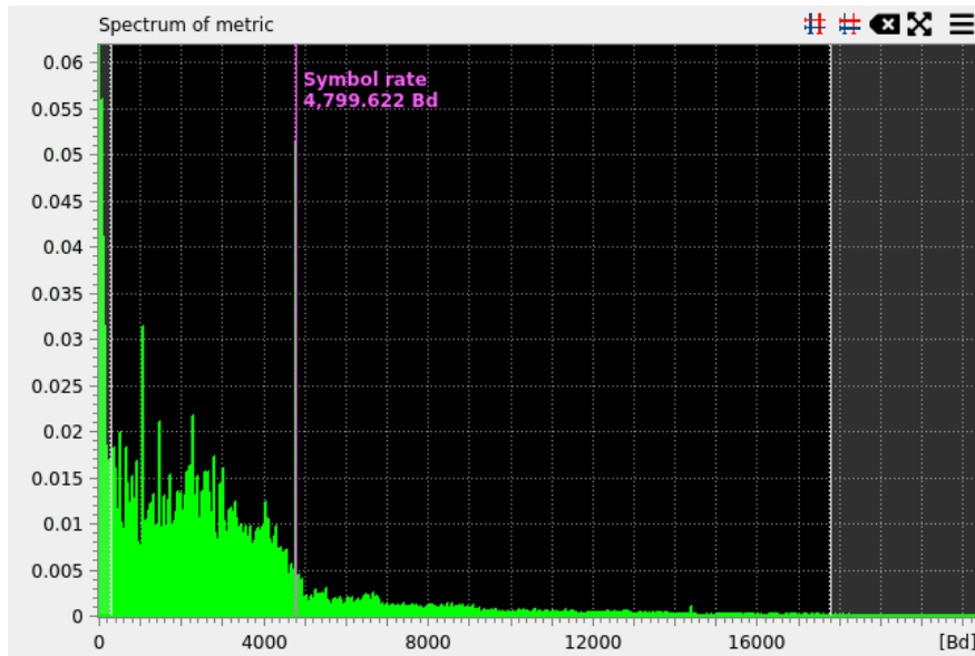
Figure 23: Spectrum for metric 'Quadrature distance' on an APCO-25 signal
