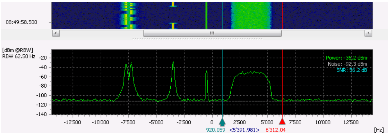
Figure 13: Spectrum/Sonogram with measurement values power, noise and SNR
