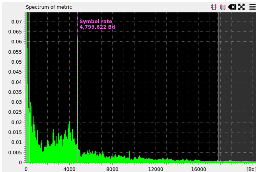
Figure 24: Spectrum for metric 'Inst. Frequency (abs of diff)' on same APCO-25 signal
