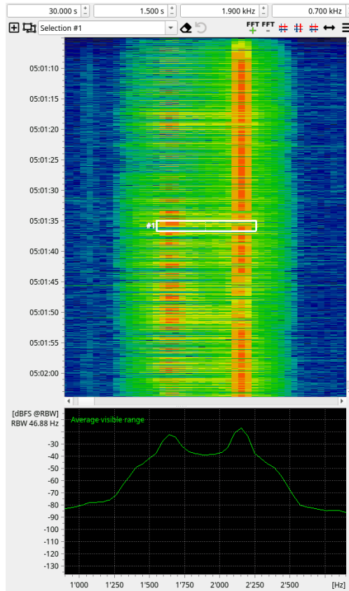
Figure 37: Input sonogram of the FSK-2 example.
