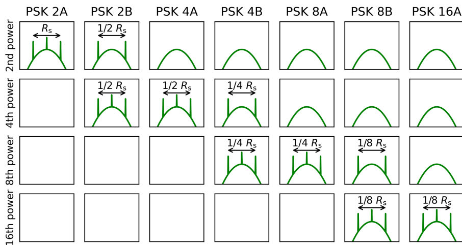
Figure 27: Expected peaks in squared signals spectra for different PSK modulation types and squaring degrees.
