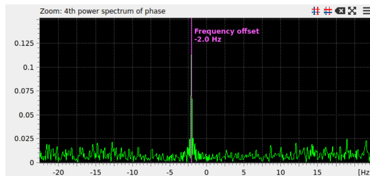
Figure 29: Zoomed: 4th power spectrum of phase.
