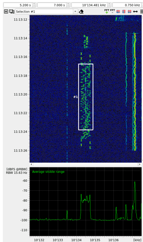
Figure 58: Input sonagram of the Multitone example.
