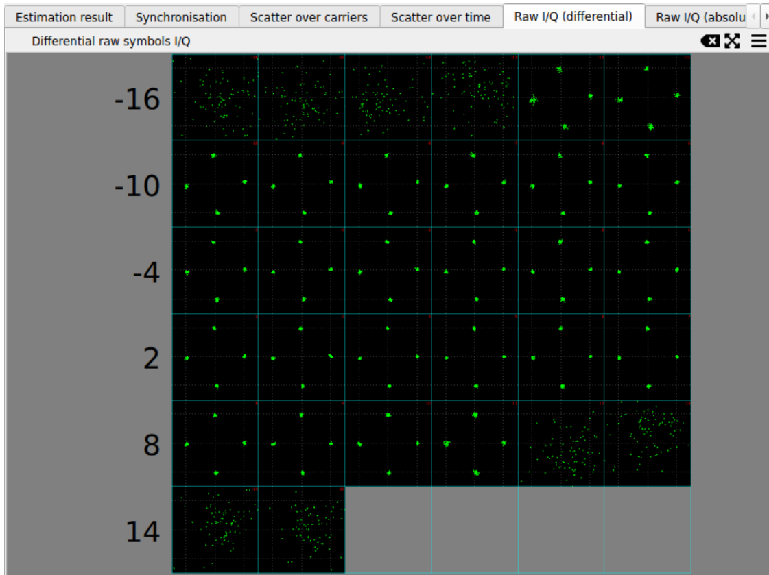
Figure 48: Example output of a multicarrier I/Q diagram of raw differential symbols
