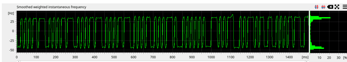
Figure 35: Smoothed weighted instantaneous frequency
