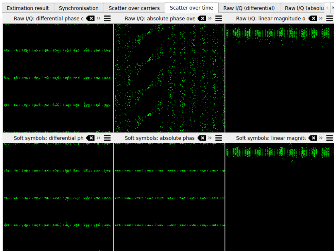
Figure 47: Example output of scatter diagrams over symbol number (i.e. time)
