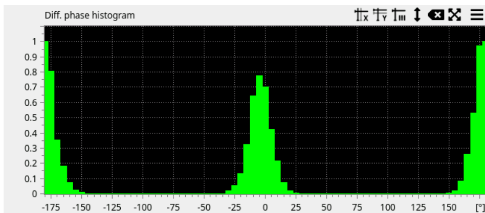
Figure 10: example histogram-plot: A3 spectrum
