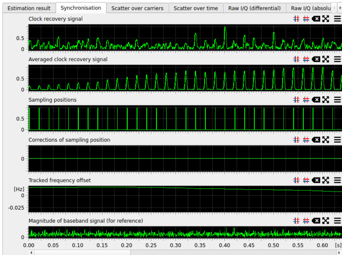
Figure 45: Verification of clock recovery.
