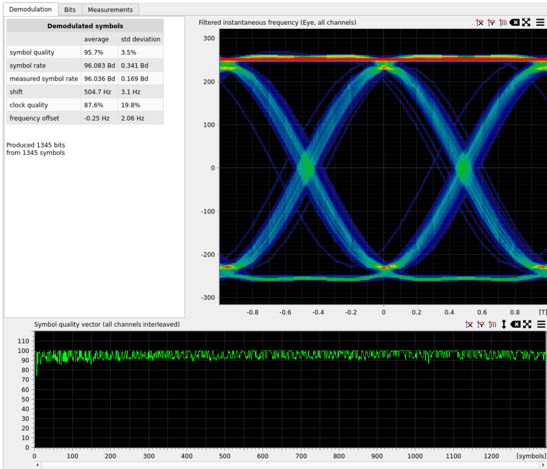
Figure 61: Demodulation output overview (FSK-2).
