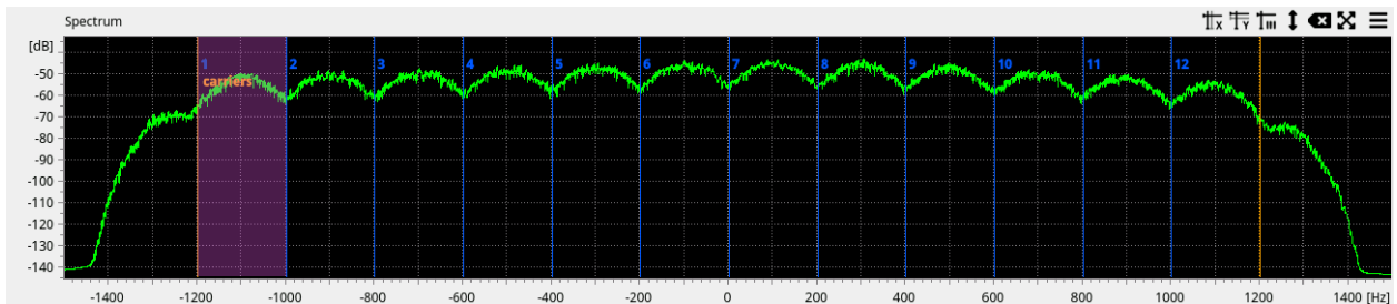
Figure 9: example frequency-plot: averaged spectrum
