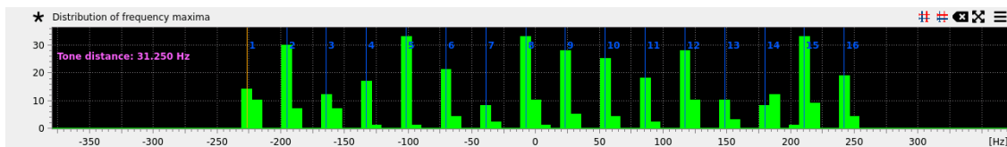
Figure 55: Distribution of frequency maxima - after doubling the DFT length once
