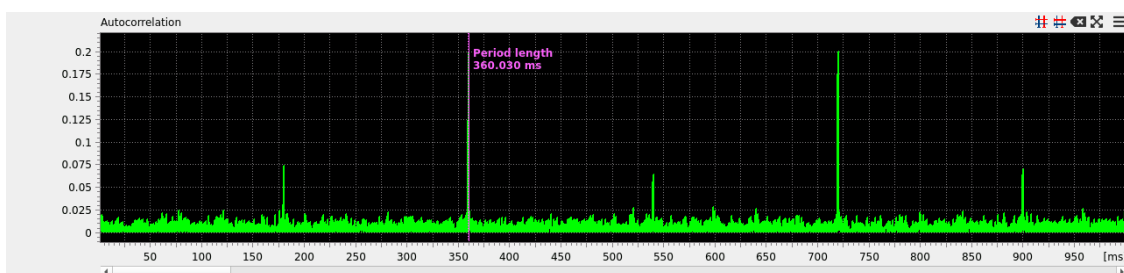
Figure 19: Example of the autocorrelation of a signal with multiple different repetitive components.
