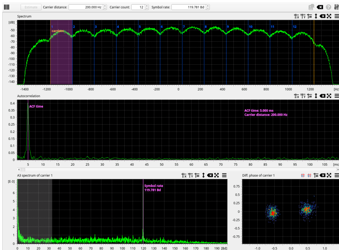
Figure 40: Multi-carrier analysis view of an example 12 carrier PSK2 signal
