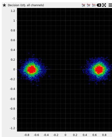
Figure 63: I/Q plot for 12-channel DPSK-2A
