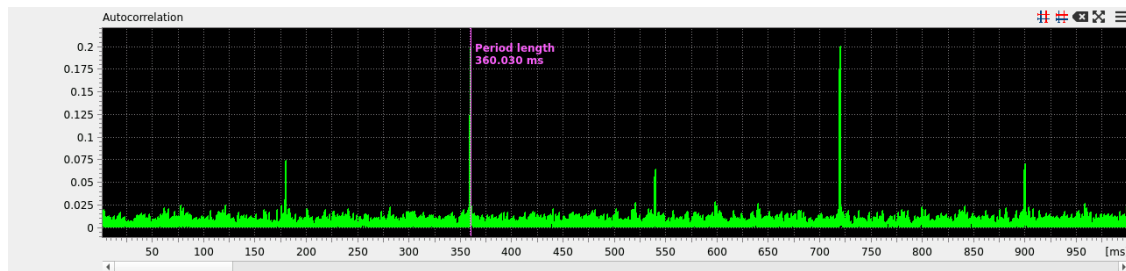
Figure 20: Example of the autocorrelation of a signal with multiple different repetitive components.
