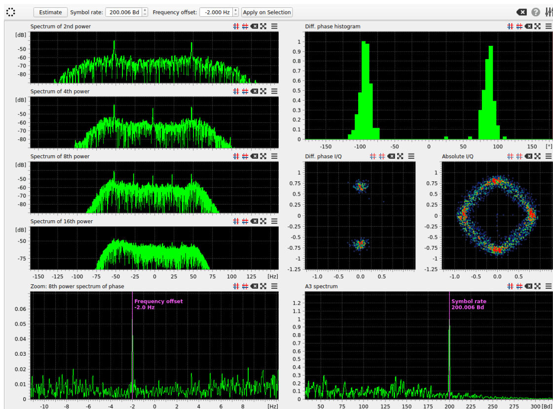
Figure 26: PSK analysis result display overview.
