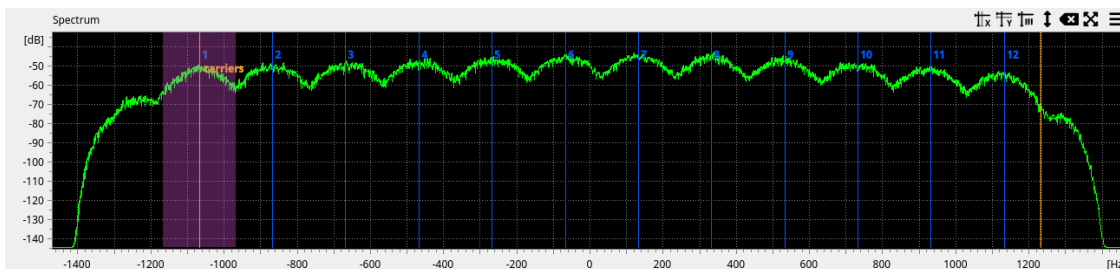
Figure 42: Averaged spectrum with markers placed on carrier frequencies.
