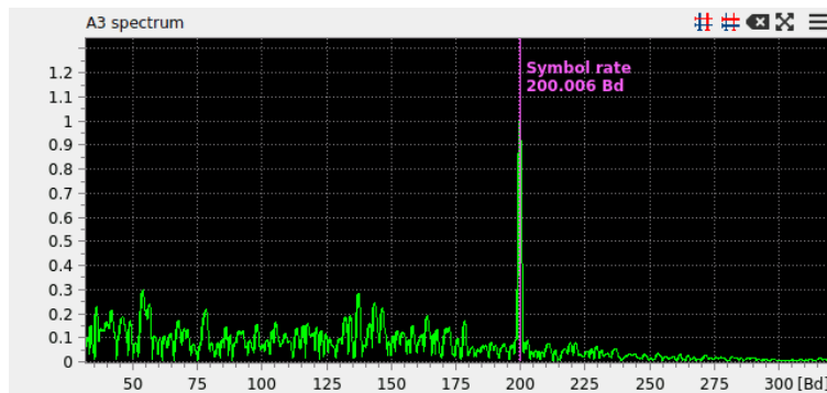
Figure 30: A3 spectrum for symbol rate estimation.
