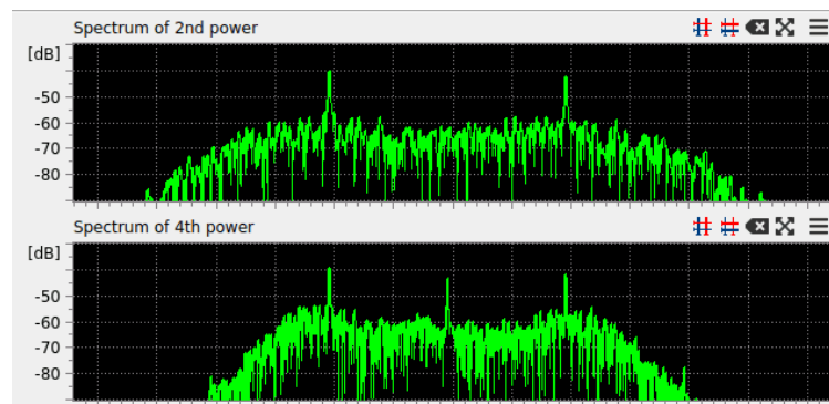
Figure 28: Spectra for one and two times squared signal (2nd and 4th power).
