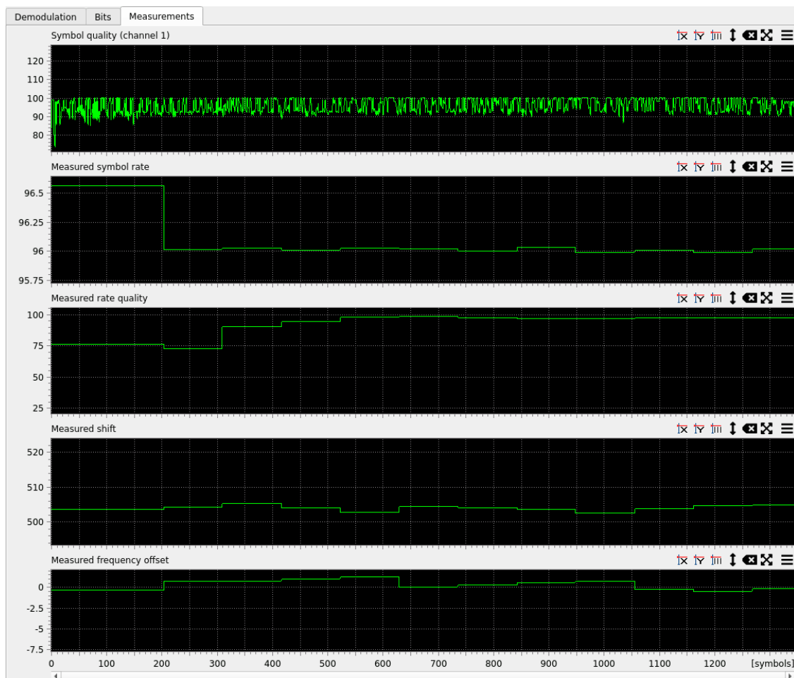
Figure 64: Measured result traces over time (for FSK-2)
