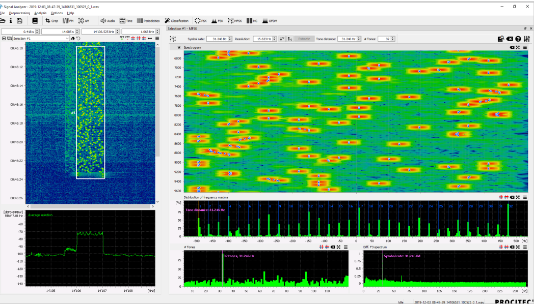
Multitone analysis: Just select the signal in the recording and you get all modulation parameters
