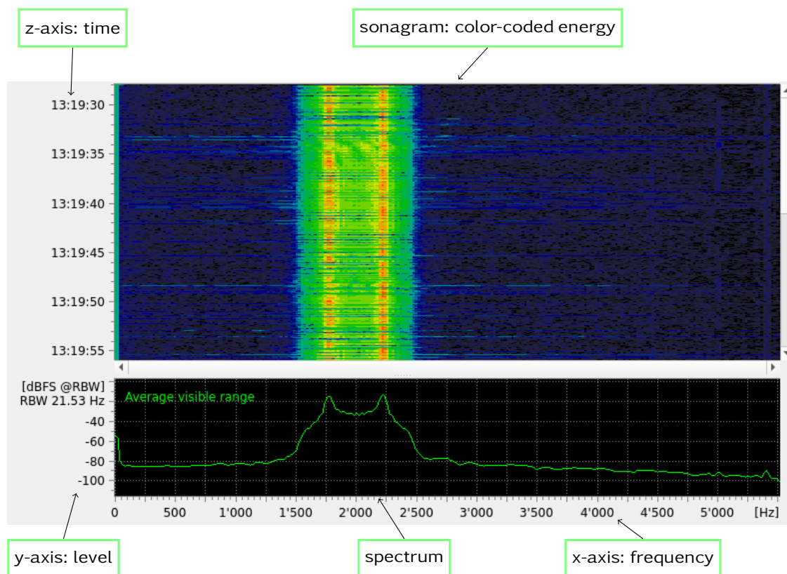
Figure 15: Spectrum/Sonagram
