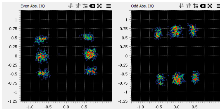
Figure 42: Absolute even (left) and odd (right) symbols
