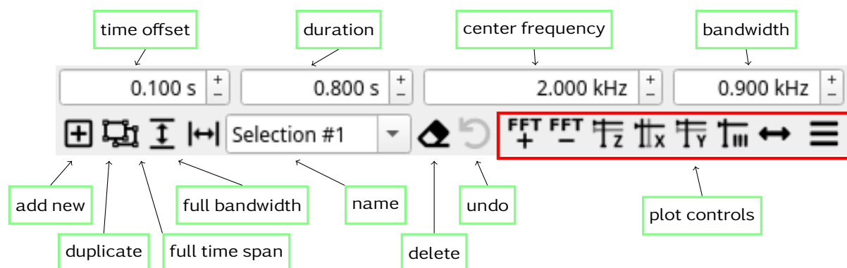
Figure 5: Input sonagram toolbars
