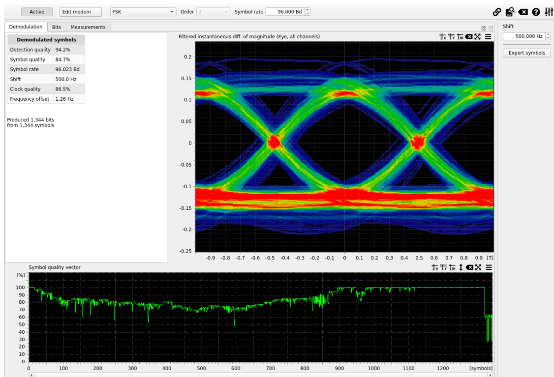
Figure 76: Demodulation output overview (FSK-2).
