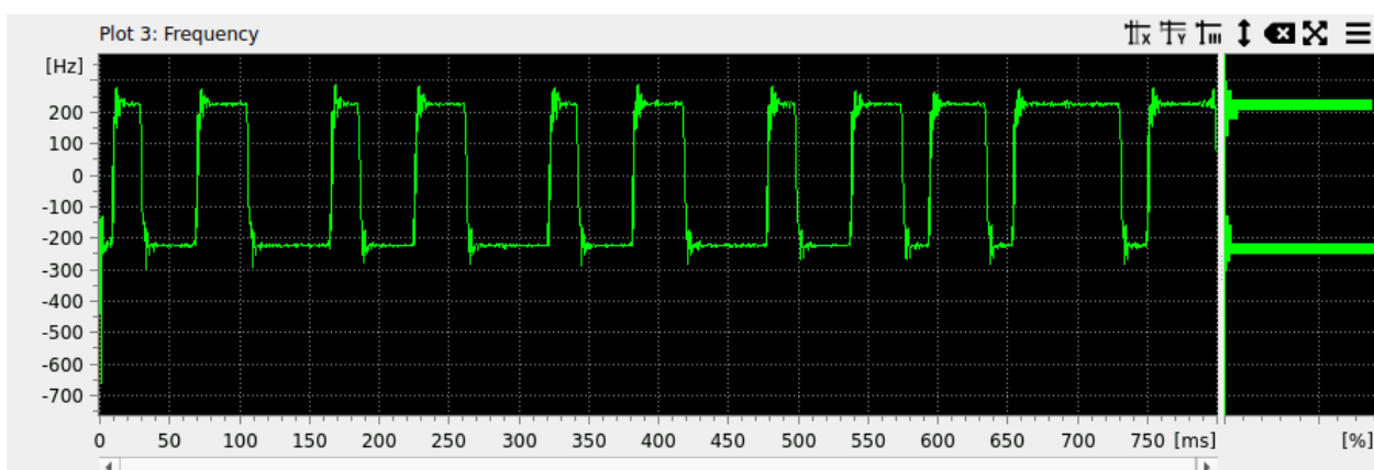
Figure 11: Time Plot
