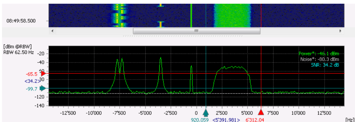
Figure 18: Spectrum/Sonogram with manually positioned Y-cursor
