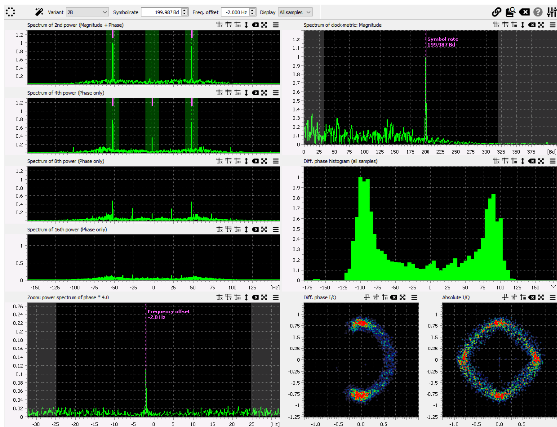
Figure 29: PSK analysis result display overview.
