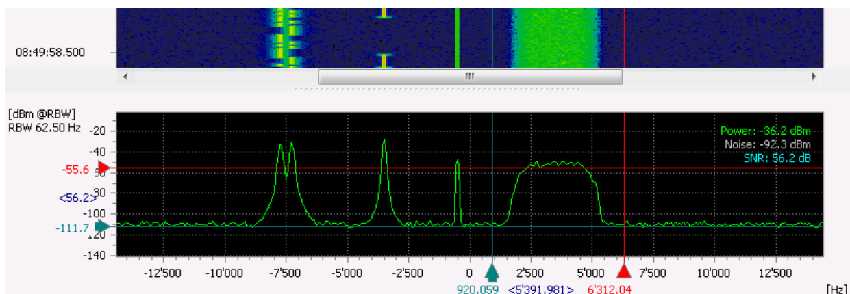
Figure 17: Spectrum/Sonogram with synchronized Y-cursor
